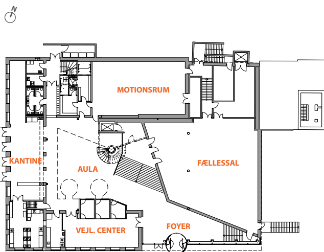
PARTERREPLAN
