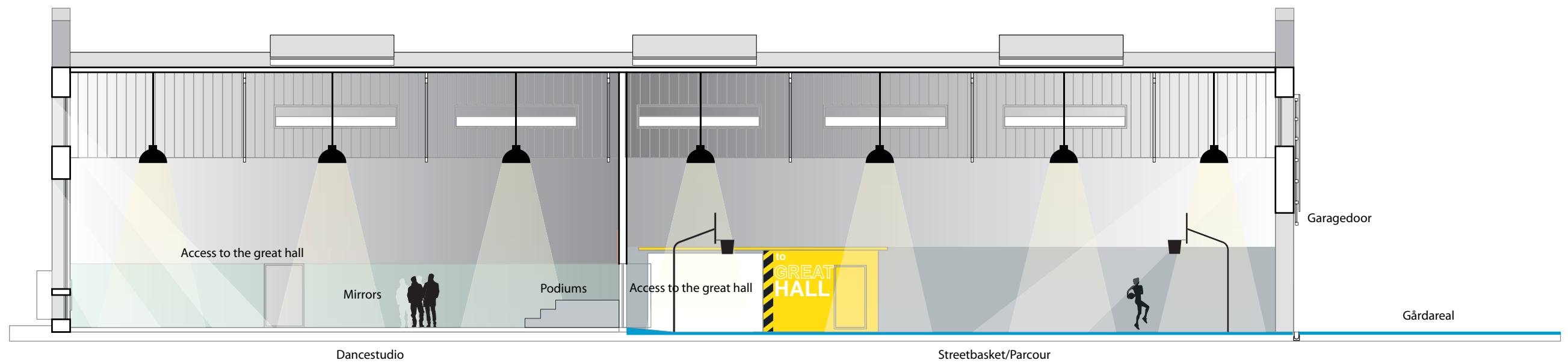
Section 1:150 Streetmekka/Small Hall
