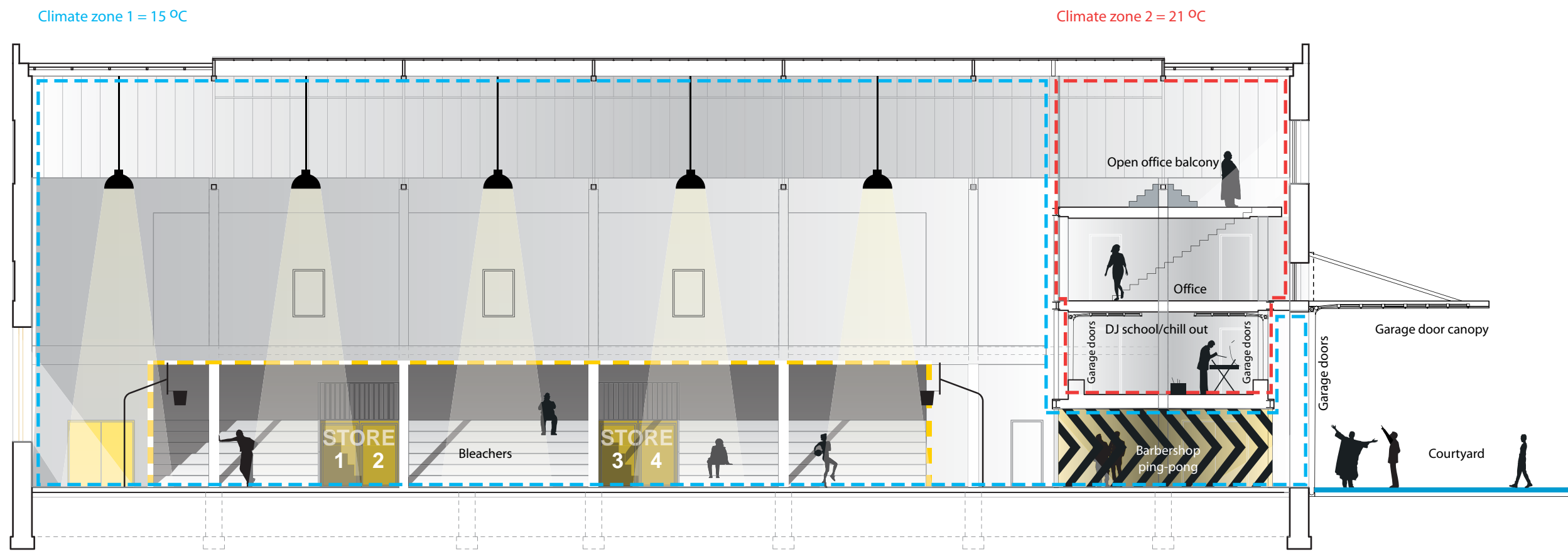
Section 1:150 Streetmekka/Great Hall
